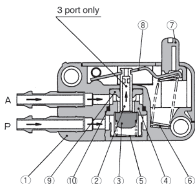
Bottom Piping
