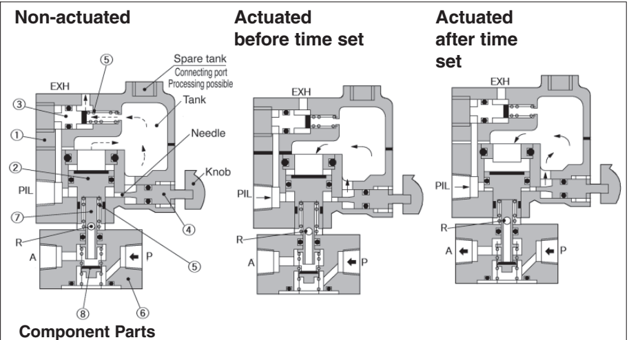
Component Parts
