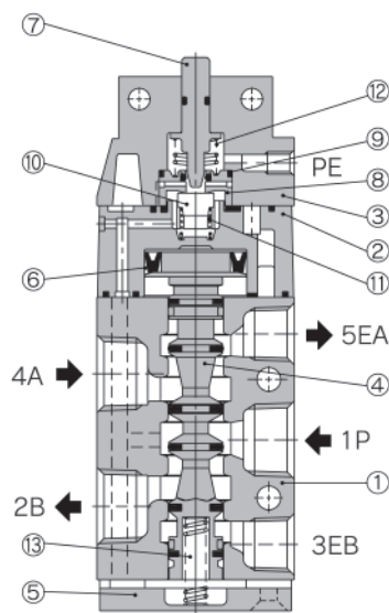
Non-actuated
