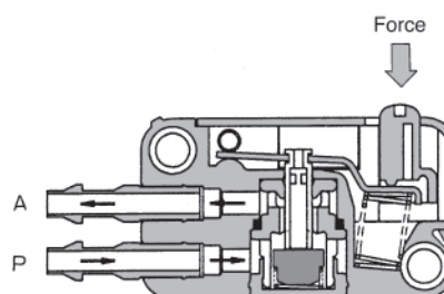
Side Piping/Actuated
