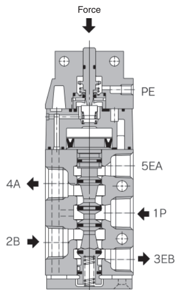
Actuated
