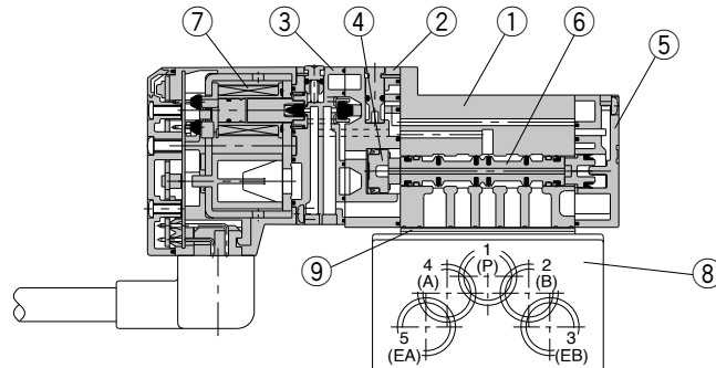
5/2 bistable
