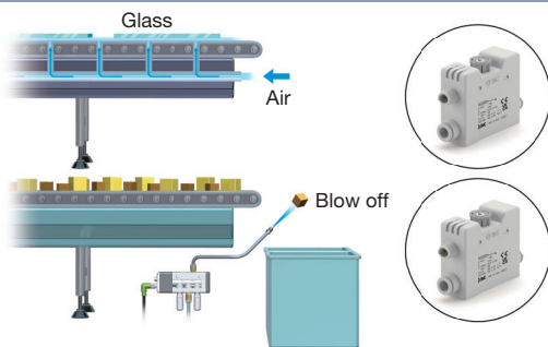
Workpiece handling
