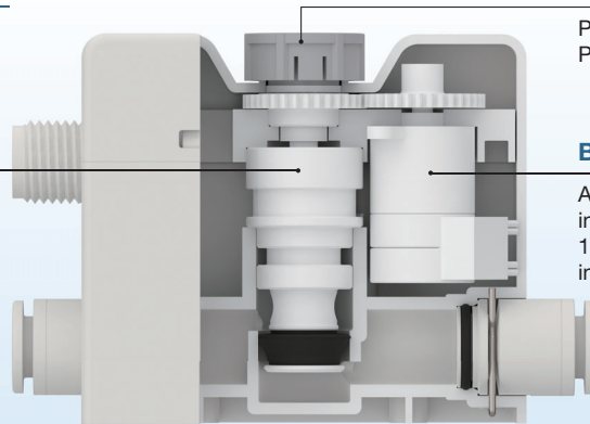
Needle valve
