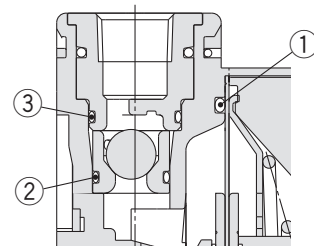
①-③: O-rings (SF7000)
