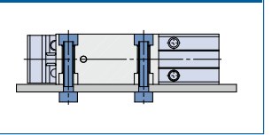
Lateral mounting (Body thread)
