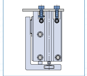
Axial mounting (Body thread)
