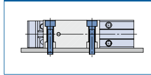
Lateral mounting (Body through-hole)
