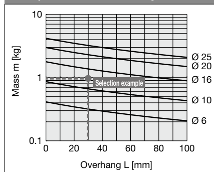
Graph 6 Load Eccentricity 200 mm
