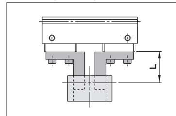
Internal gripping state
