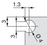
Dimensions of auto switch mounting groove
