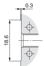
Section A details
