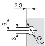
Dimensions of auto switch mounting groove
