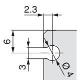
Dimensions of auto switch mounting groove
