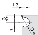
Dimensions of auto switch mounting groove
