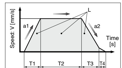
<Speed-Work load graph> (LEFSW25/Battery-less absolute)
