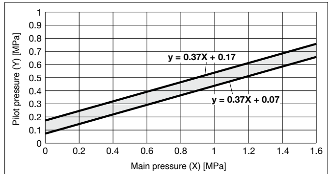
JSB44-ST25A□-3S
