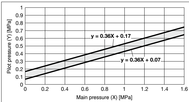
JSB54-ST32A□-4S
