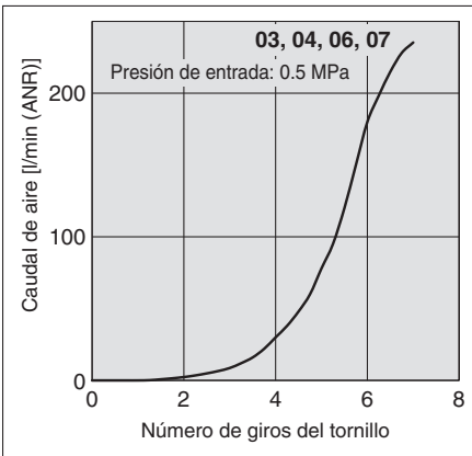
JASV-LE□□-□01□ OUT-EXH. Caudal
