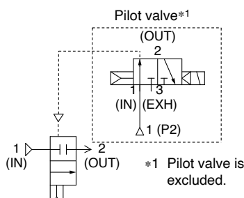
Air operated type
