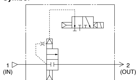
Solenoid valve type
