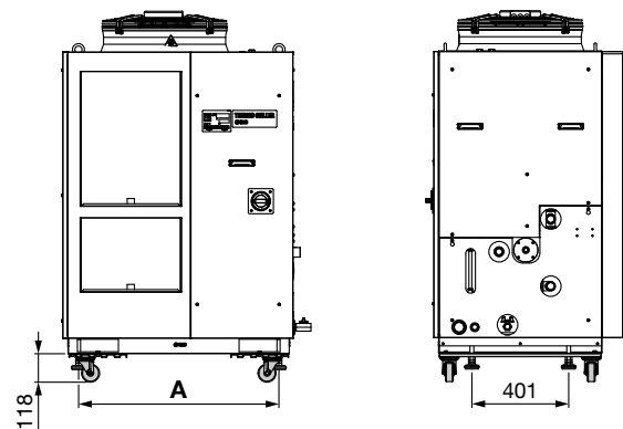
Fig. 1 Mounting view
