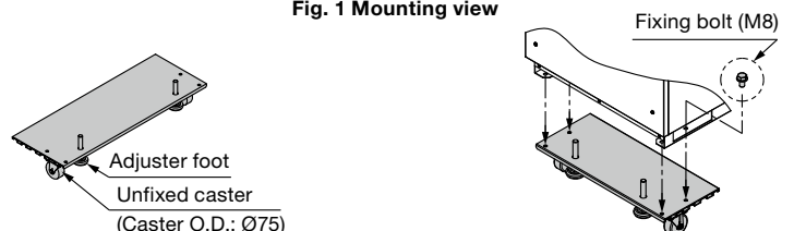
Fig. 1 Mounting view
