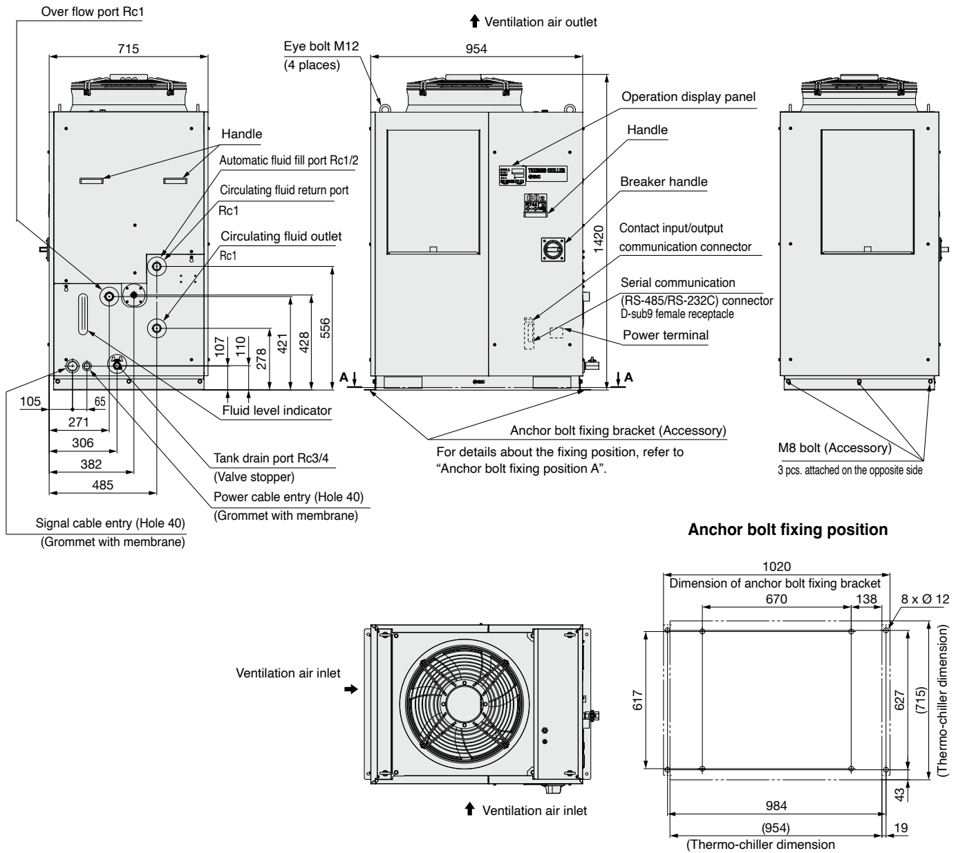
View A
