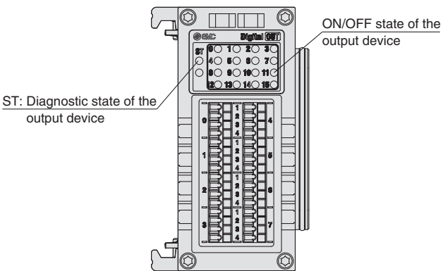
EX600-DY□F
