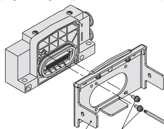
Valve plate
