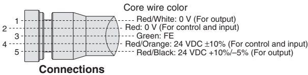
Connections
