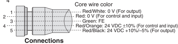
Connections
