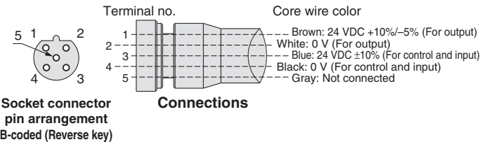
Socket connector pin arrangement B-coded (Reverse key)
