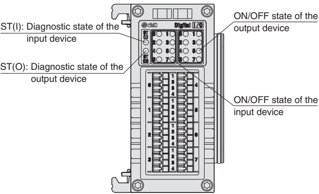
EX600-DM□F
