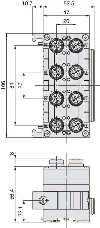
EX600-DX□D
