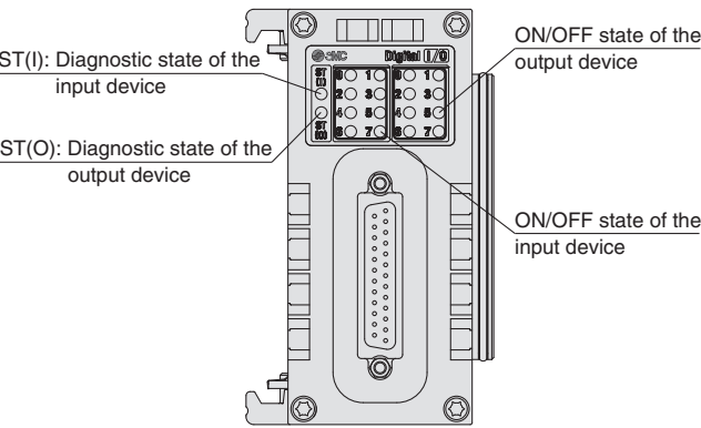
EX600-DM□E
