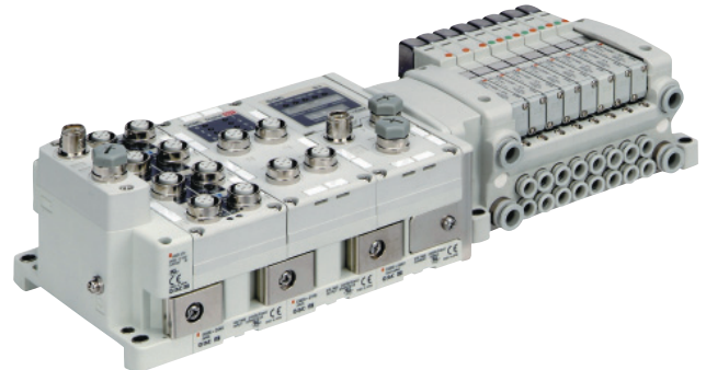
VQC1000/2000/4000/5000 Series
