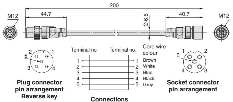
EX9-AC002-3
