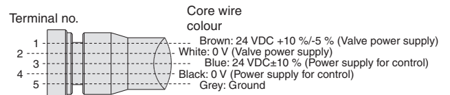
Connections (PROFIBUS DP, EtherNet/IP™)
