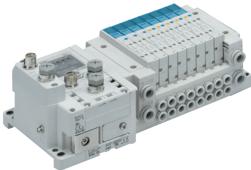
SY3000/5000/7000 Series
