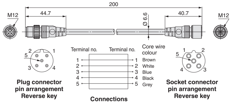
EX9-AC002-2
