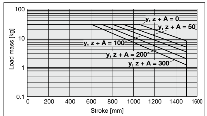
[Graph 6] Allowable load mass by stroke \varnothing 32
