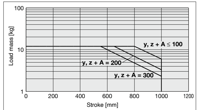
[Graph 6] Allowable load mass by stroke \varnothing 32
