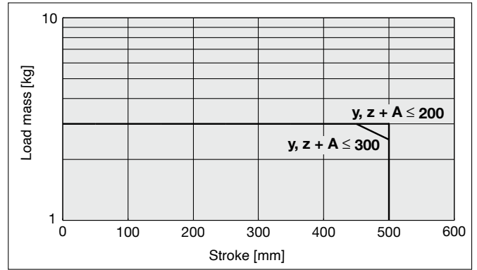
[Graph 4] Allowable load mass by stroke \varnothing 20
