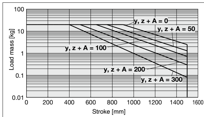
[Graph 7] Allowable load mass by stroke \varnothing 40
