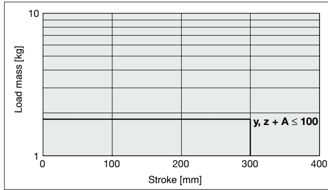
[Graph 3] Allowable load mass by stroke \varnothing 15
