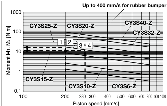
[Graph 9] Allowable moment
