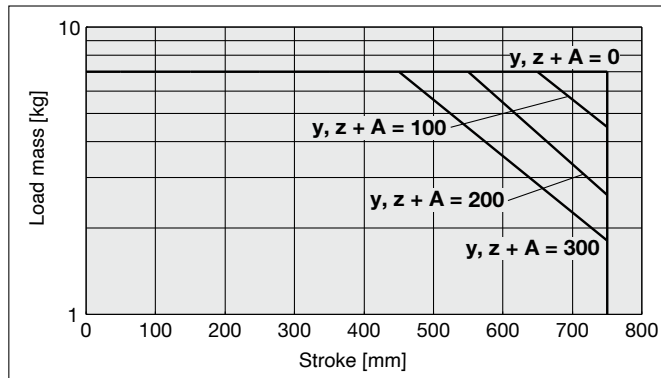
[Graph 5] Allowable load mass by stroke \varnothing 25
