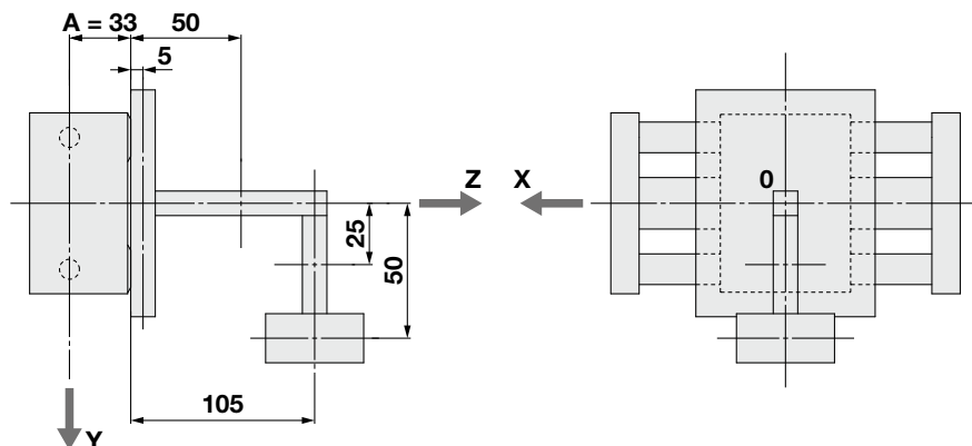
Mass and centre of gravity of the load
