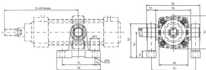
Centre trunnion
