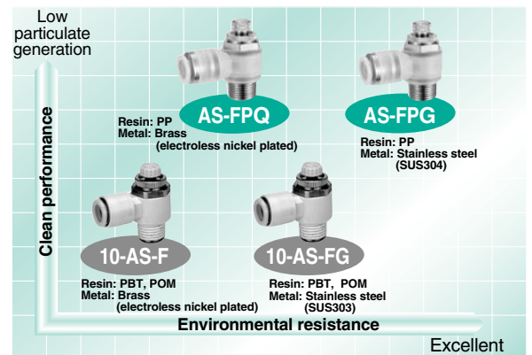
Series AS-FPG Stainless steel (SUS304)
