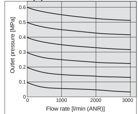
ARG40(K)-B Rc1/2
