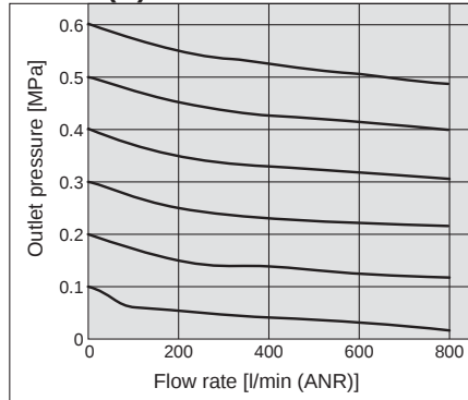
ARG20(K)-B Rc1/4
