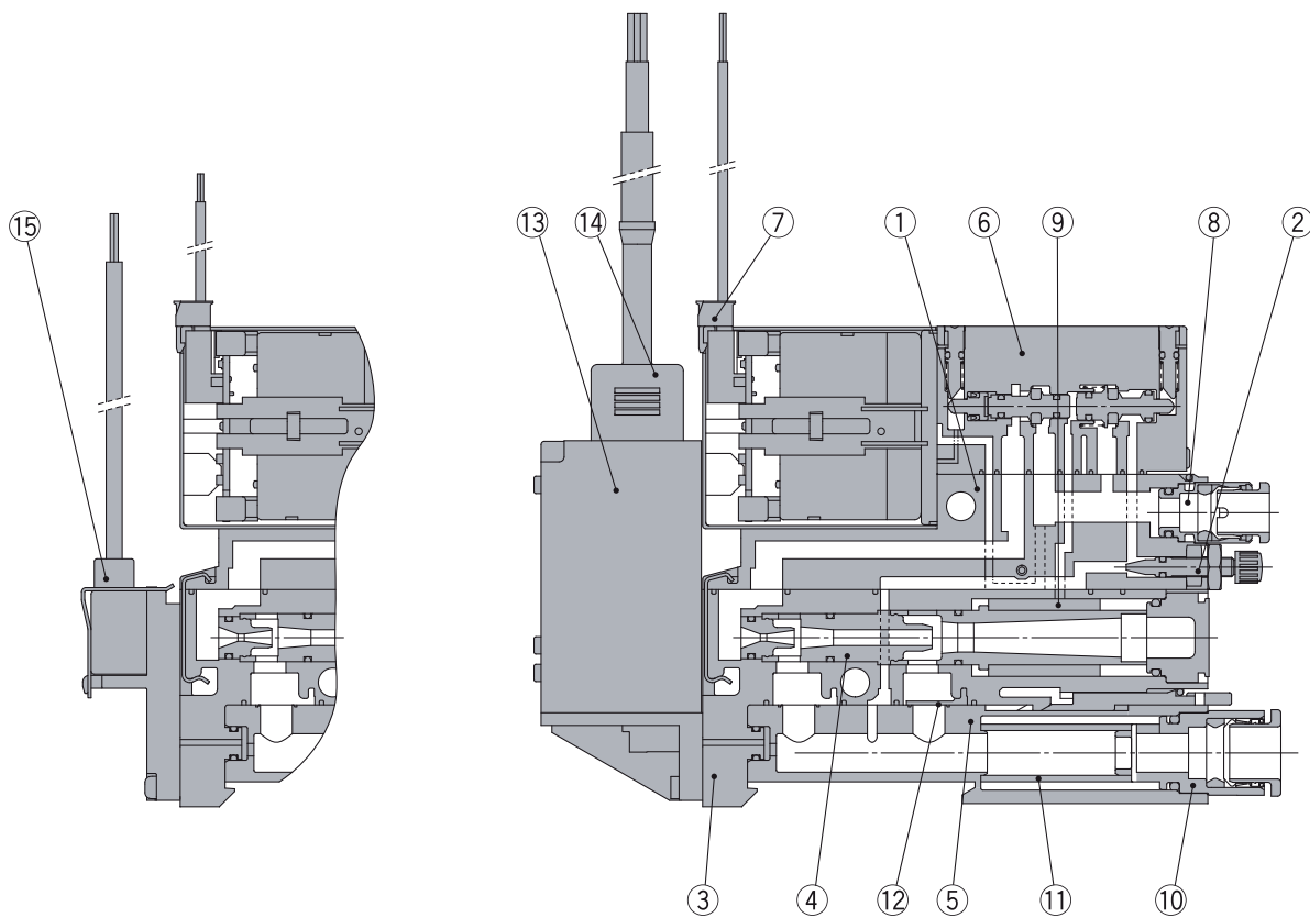
With Pressure Sensor
