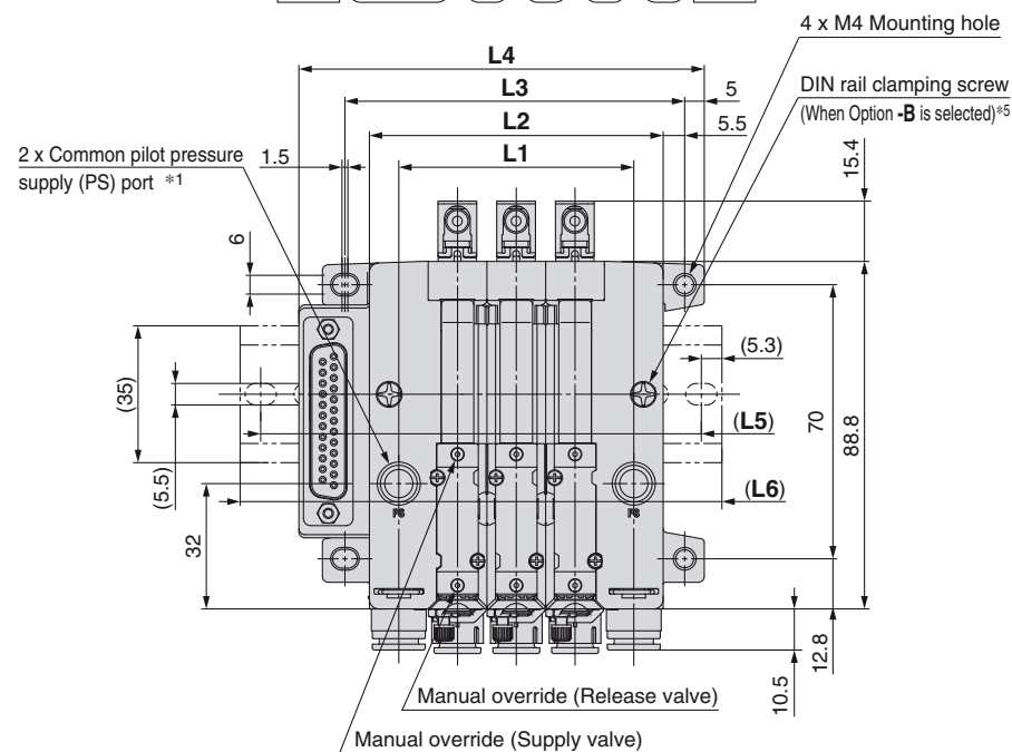
DIN rail mounting bracket Option symbol (-B)*5
