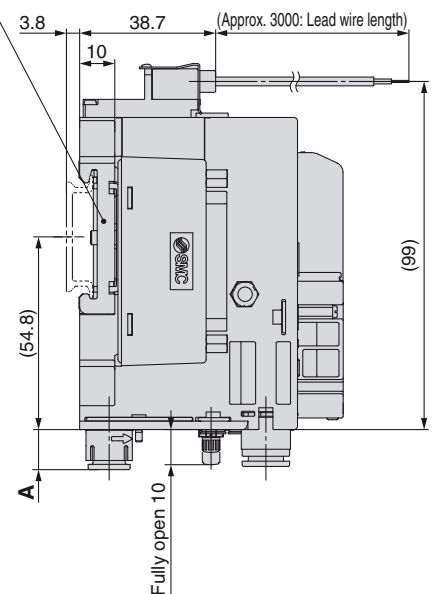
DIN rail mounting bracket Option symbol (-B)*5
