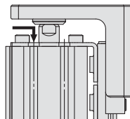
(2) When mounting an auto switch into the groove from the top (When mounting an auto switch into the groove from the top after installation)
