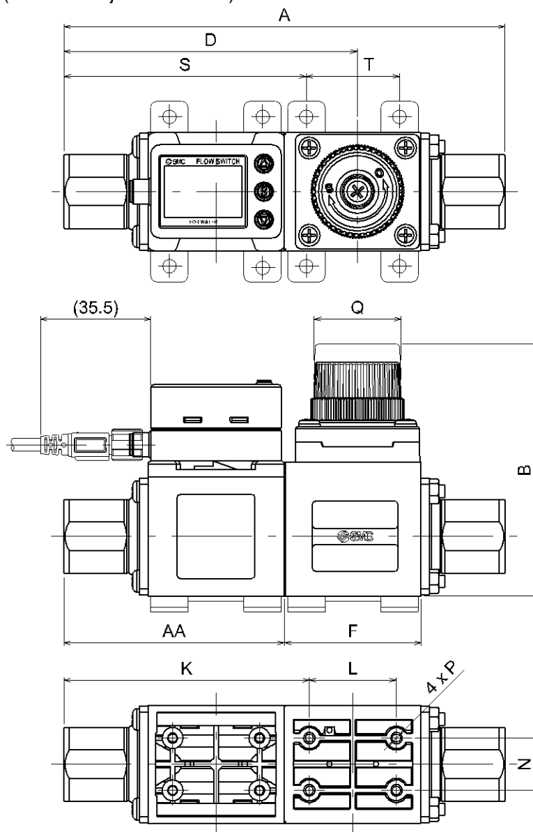
Basic type and flow adjustment valve
