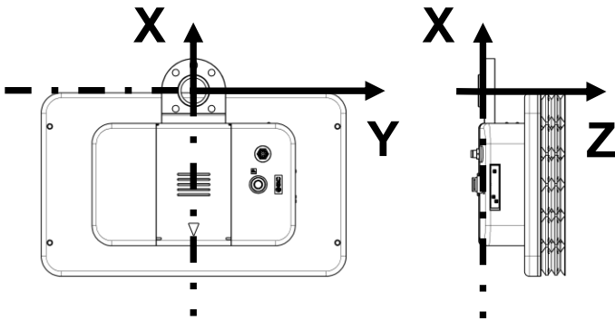
Fig 4. Offset flange
