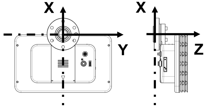
Fig 5. Offset flange + Flange U
