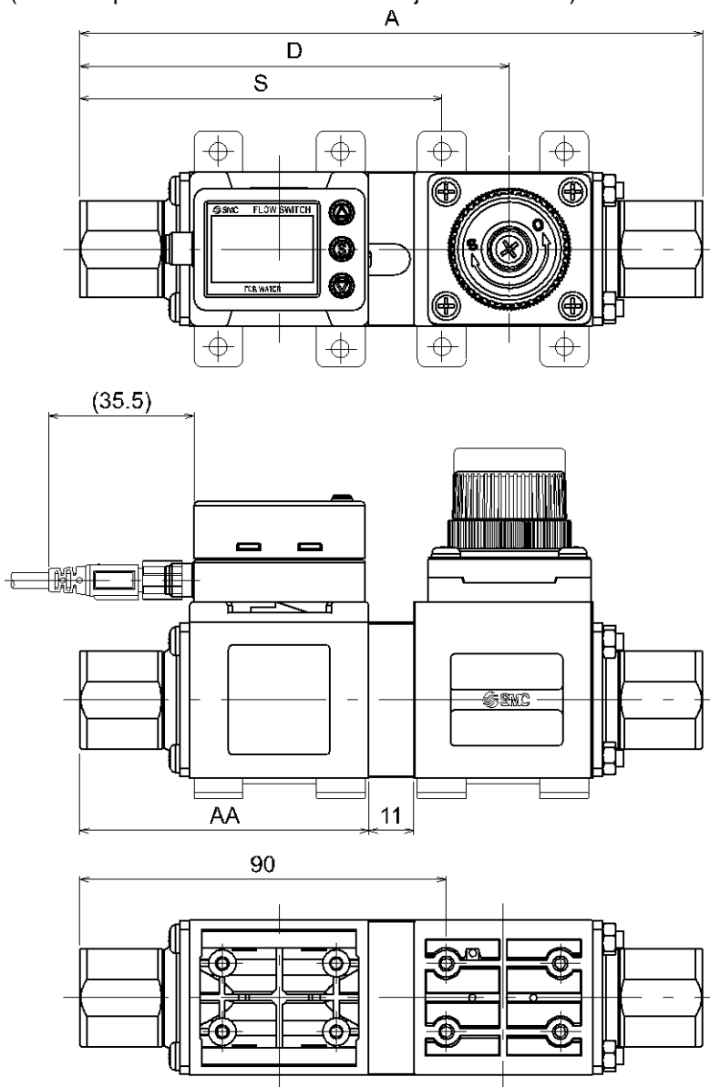
Basic type and flow adjustment valve and temperature sensor
