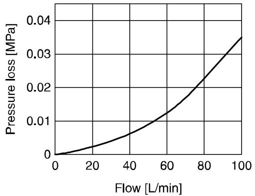
PF3W711 (Metal attachment)
