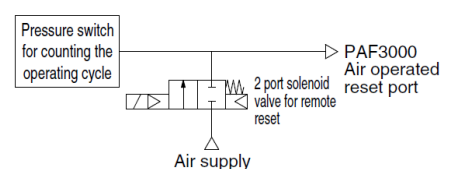
Circuit example (3)
