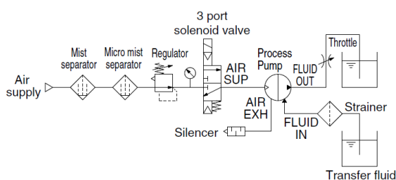
Circuit example (1)
