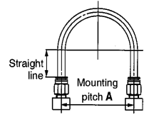
Figure 1 Recommended piping
