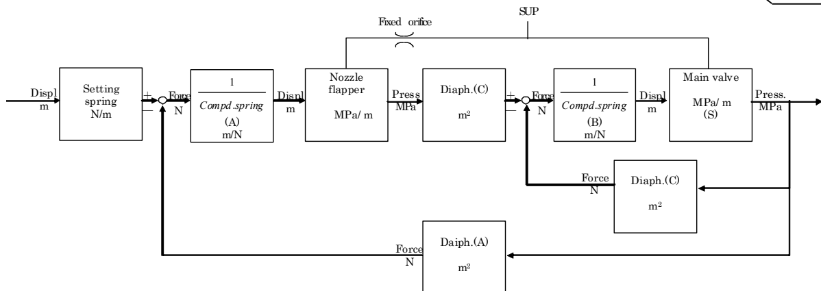
Block diagram
