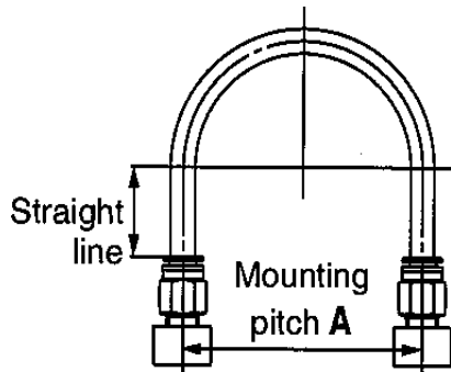
Figure 1 Recommended piping
