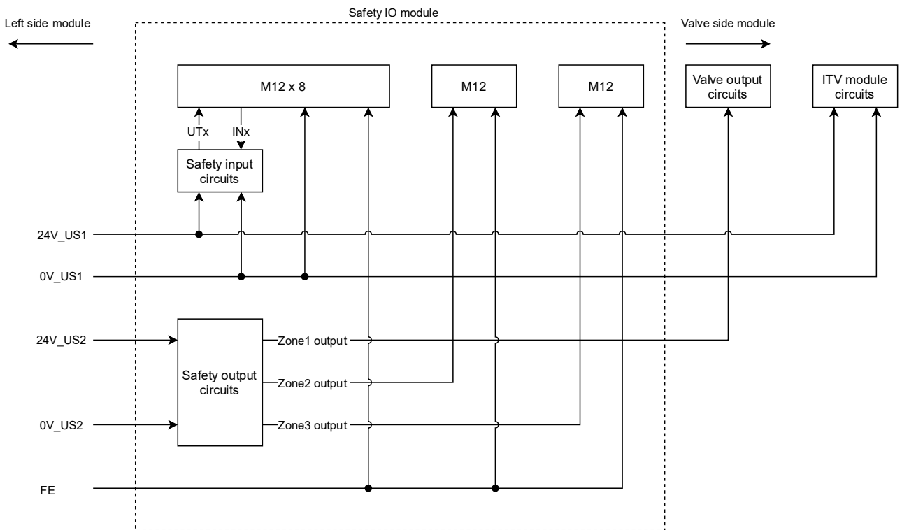
Fig. 5.4-2 EX600-FVC2
