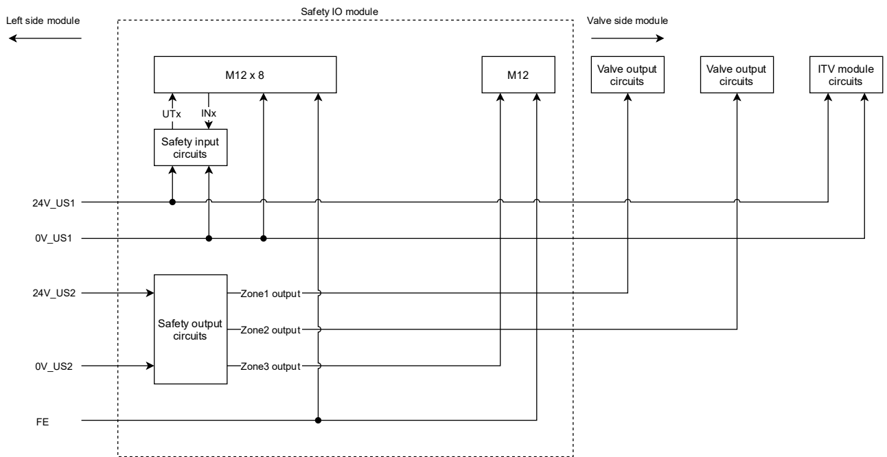
Fig. 5.4-4 EX600-FVC4
