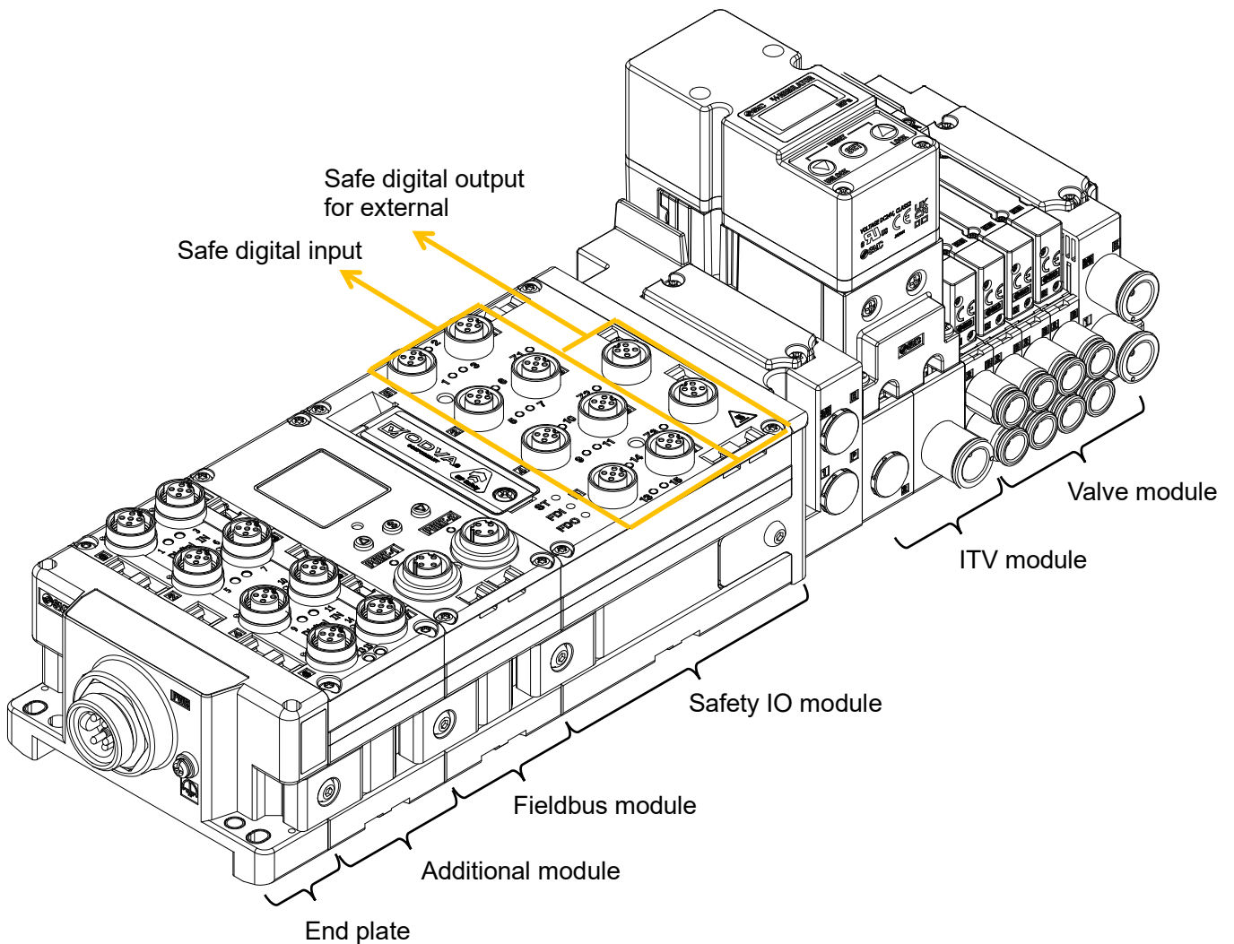
Fig. 2.3-1 Product structure: EX600-FVC#
