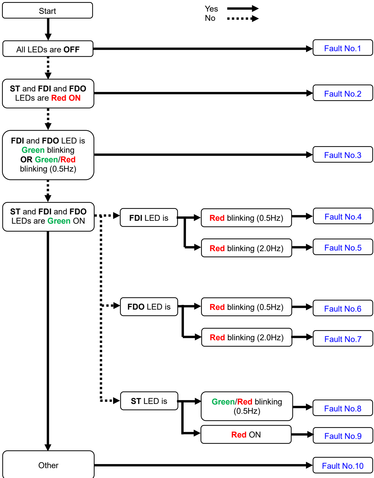
Fig. 6.2-1 Troubleshooting
