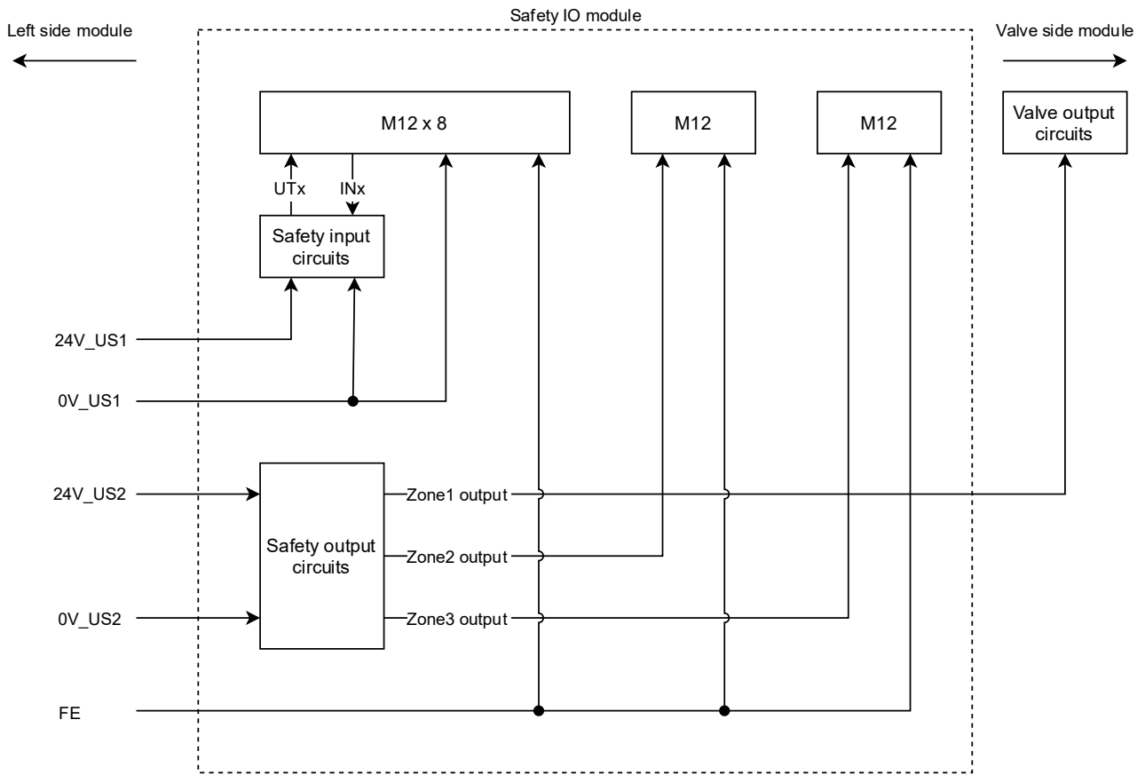
Fig. 5.4-1 EX600-FVC1
