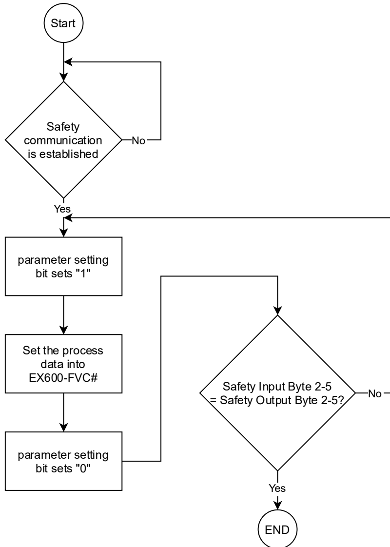
Fig. 4.4-1 Flow chart
