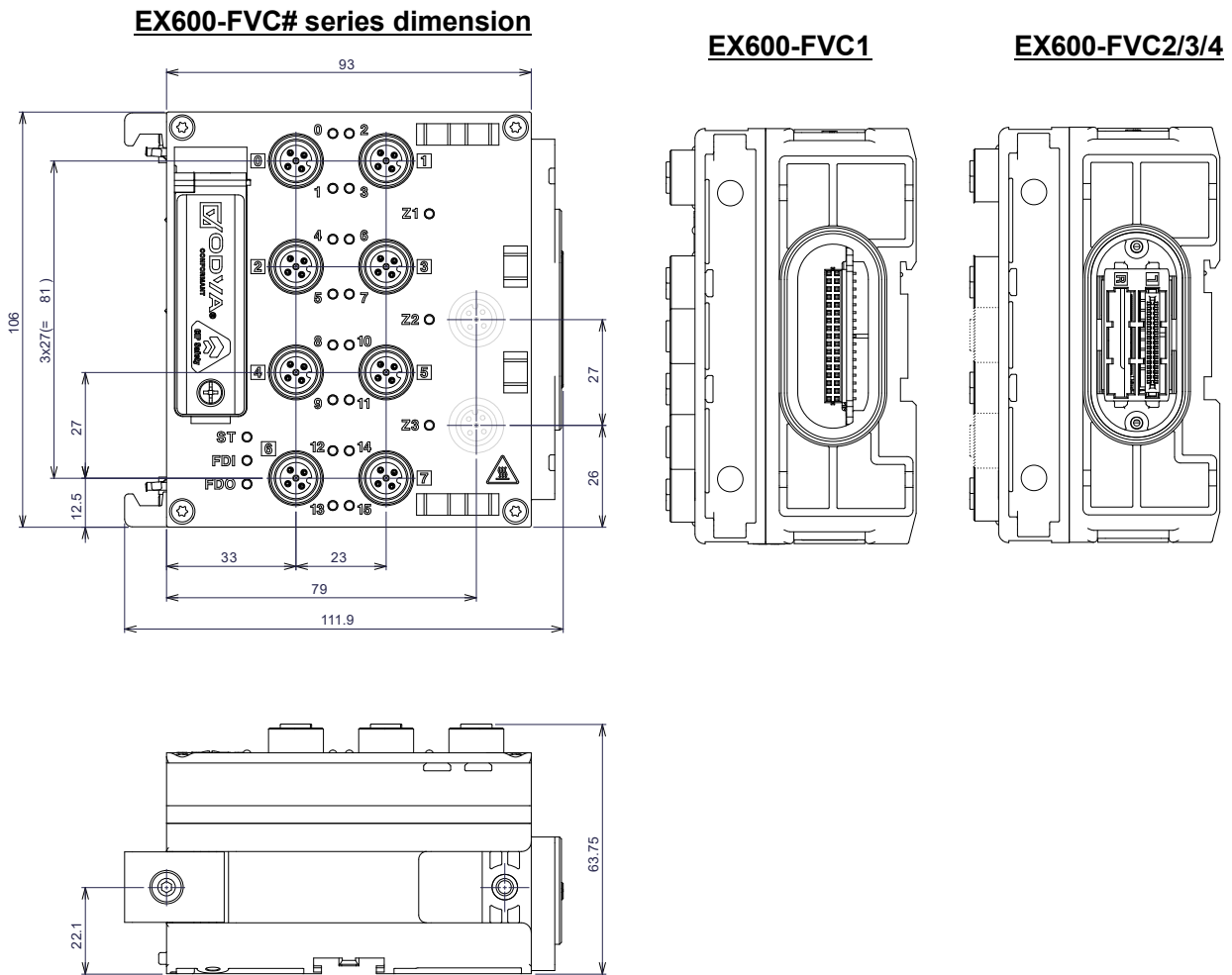
Fig. 3.2-1 Dimension: EX600-FVC# series
