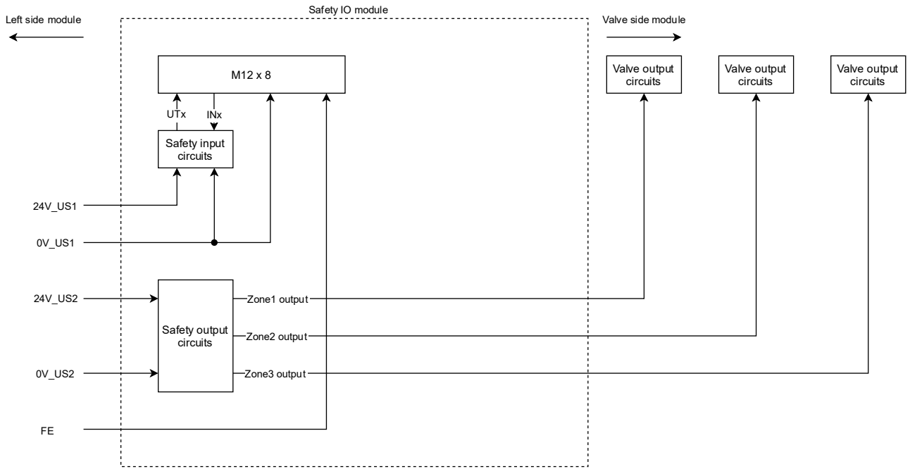
Fig. 5.4-3 EX600-FVC3
