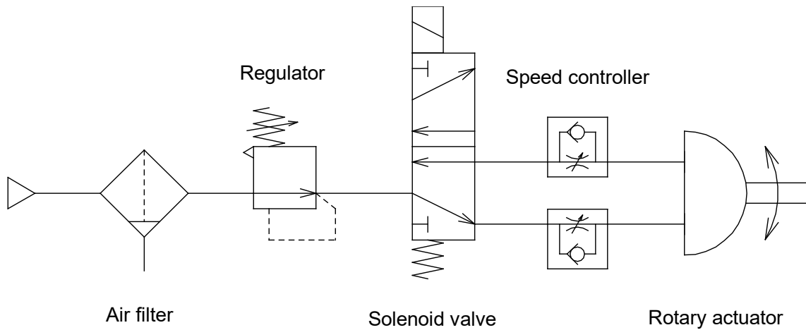
Figure 2. Basic circuit
