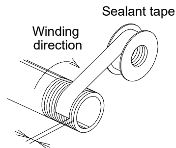
Expose approx. 2 threads Figure 8. Wrapping of pipe tape
