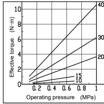
Graph 1. Effective torque
