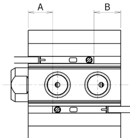
Fig. 4 Appropriate mounting position of auto switch
