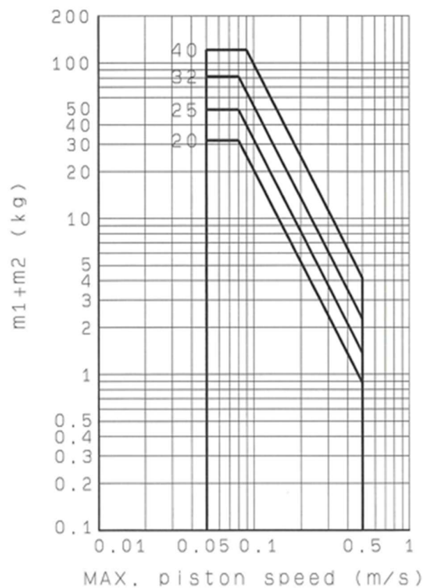
Fig.3 Operating range and kinetic energy
