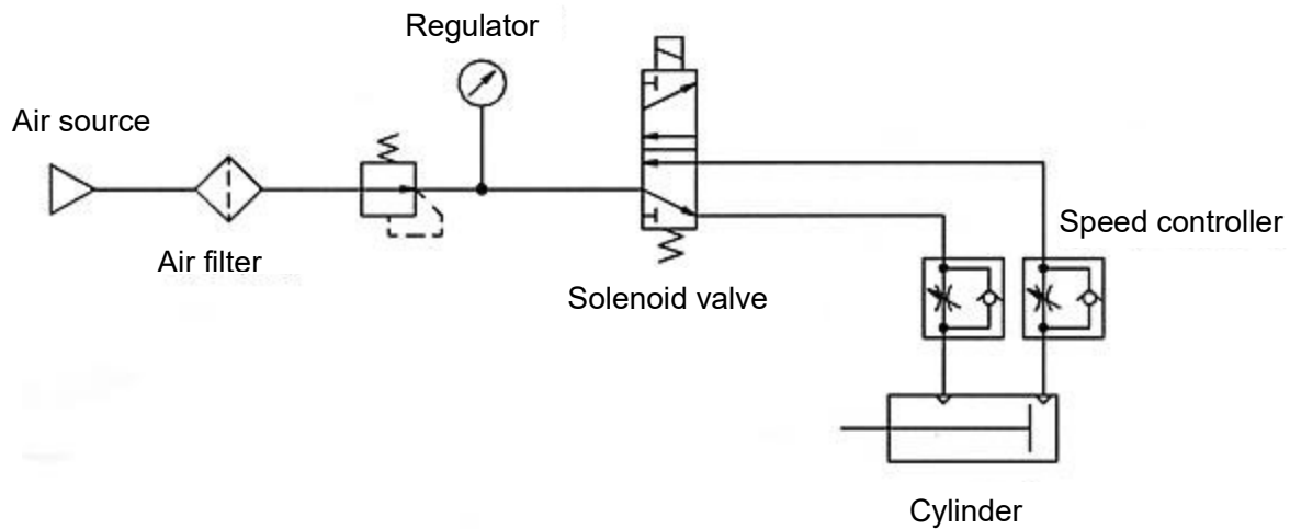
Fig. 12 Air circuit
