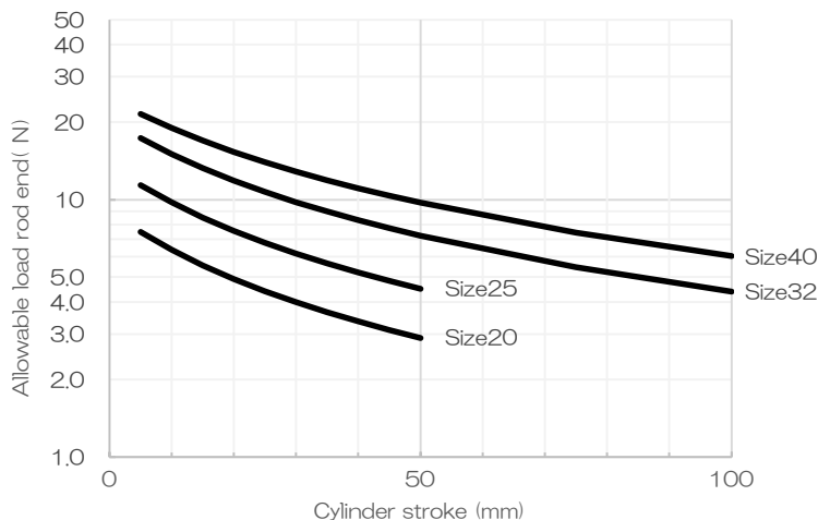
Fig.1 Allowable lateral load at rod end
