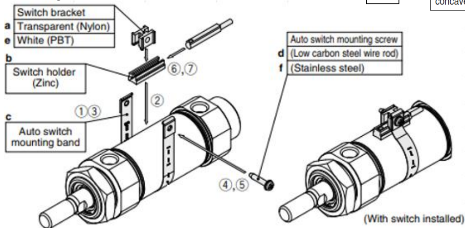
Fig. 4 Mounting and movement of the auto switch
