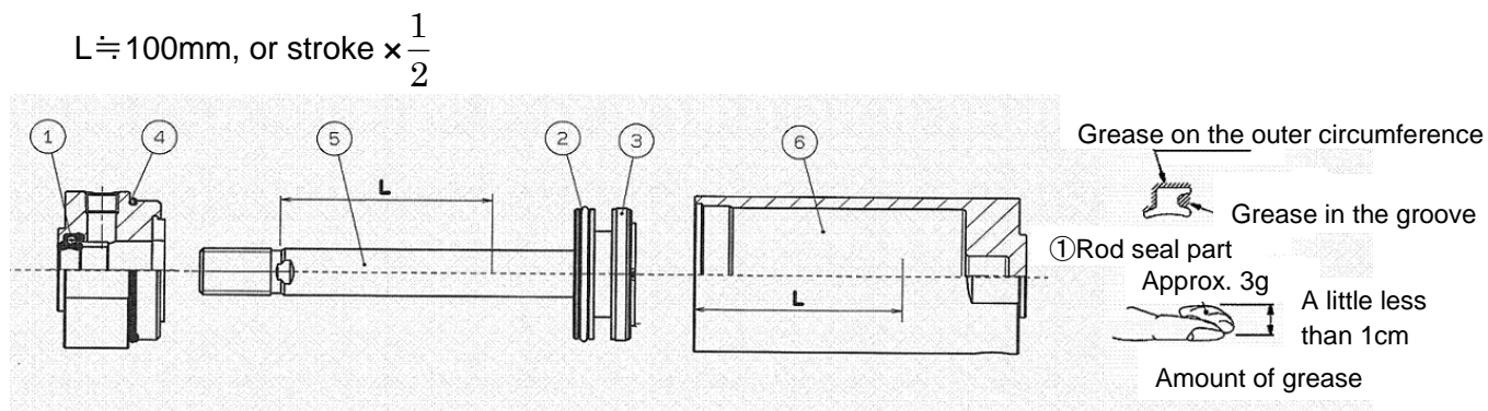
Fig. 5 Position for application of grease
