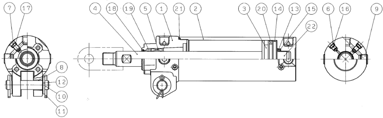
Fig. 9 Clamp cylinder construction
