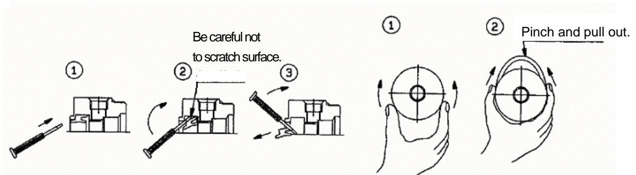
Fig. 3 How to remove rod seal
