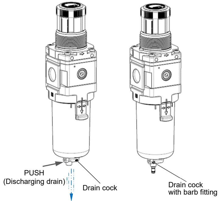
AWM30-D/ AWM40-D: Drain cock/ With barb fitting (push type) (Polycarbonate bowl/ Nylon bowl)
