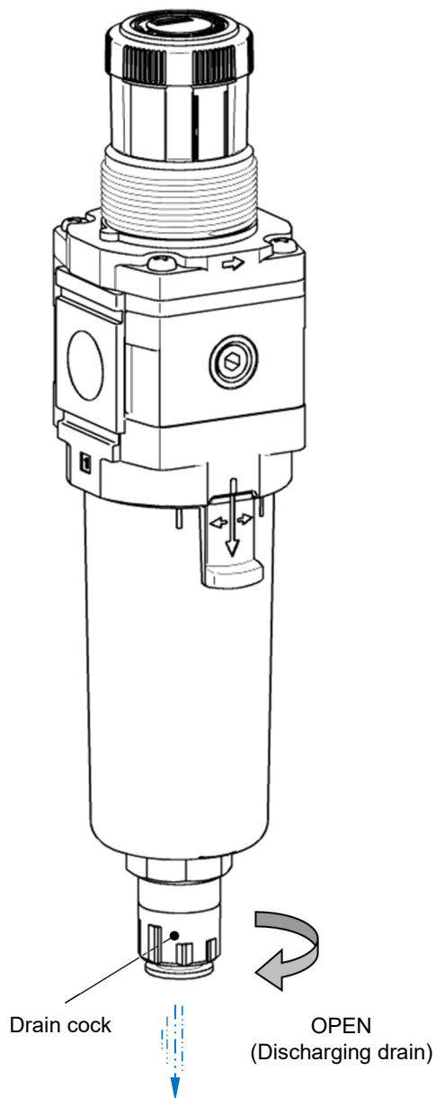
AW30-D/ AW40-D/ AW60-D: Auto drain
