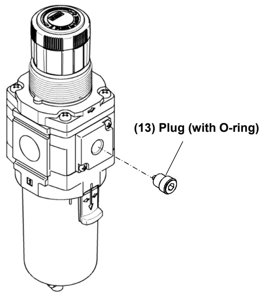
Product (AW20K-D / AW30K-D / AW40K-D/ AW60K-D)
