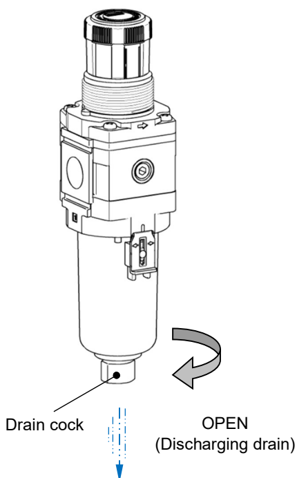
AW30-D/ AW40-D/ AW60-D: Drain cock (rotation type) (Metal bowl/ Metal bowl with level gauge)
