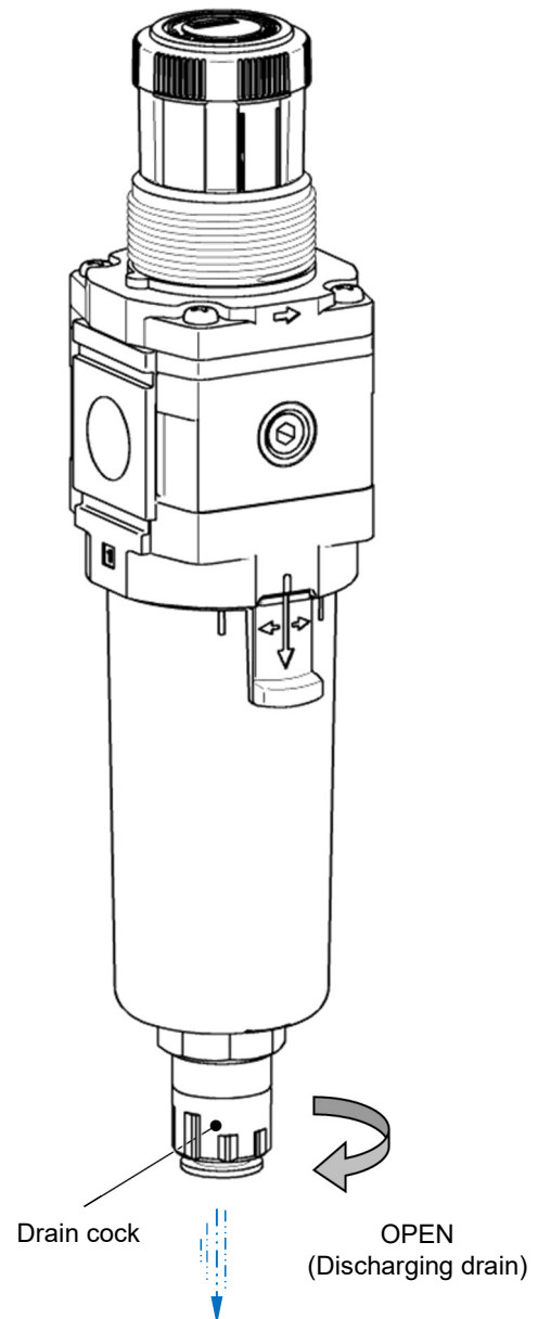
AW30-D/ AW40-D/ AW60-D: Auto drain
