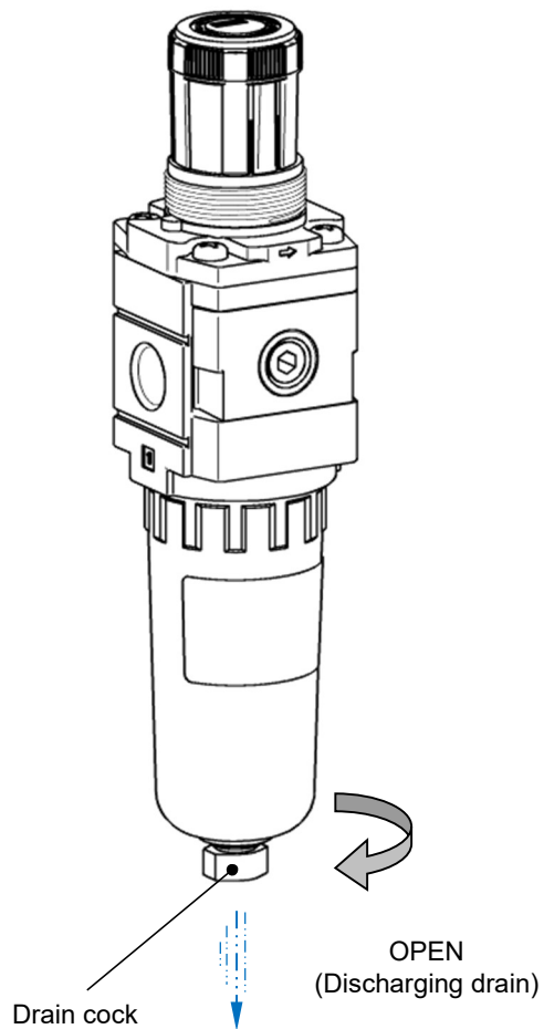
AW20-D: Auto drain
