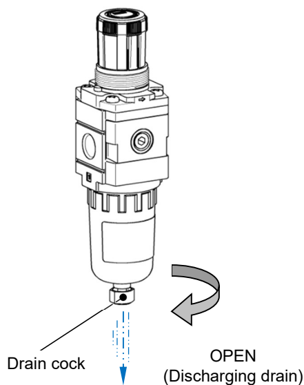
AW20-D: Drain cock (rotation type) (Polycarbonate bowl/ Nylon bowl)
