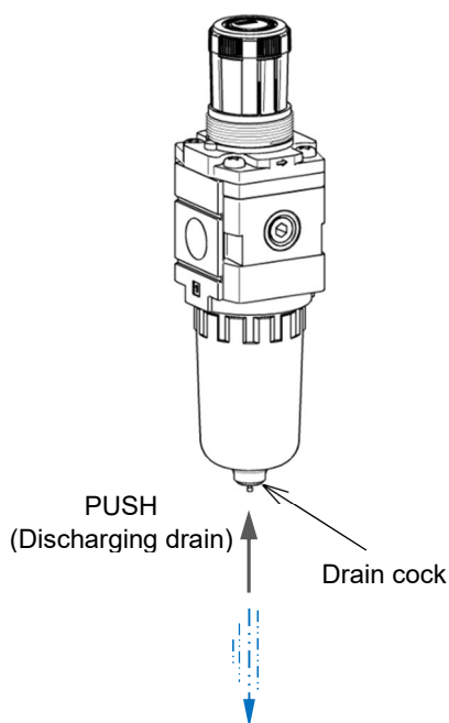
AW20-D: Drain cock (push type) (Metal bowl)
