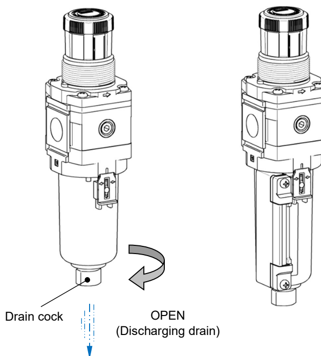
AW30-D/ AW40-D/ AW60-D: Drain cock (rotation type) (Metal bowl/ Metal bowl with level gauge)
