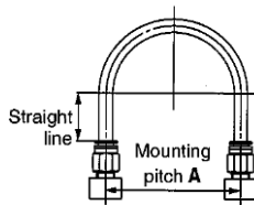
Figure 1 Recommended piping
