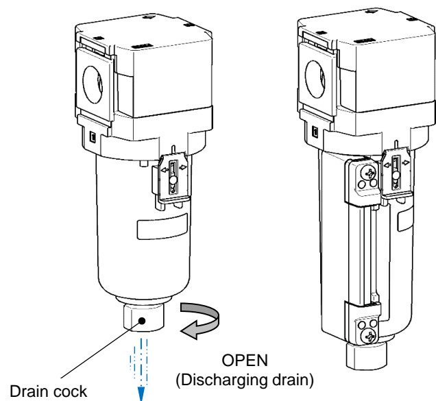
AFD30-D/ AFD40-D: Drain cock (rotation type) (Metal bowl / Metal bowl with level gauge)
