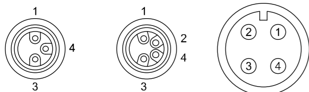
M8-3 pin connector M8-4 pin connector M12-4 pin connector
