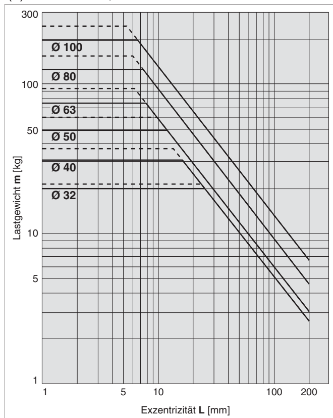
(7) Max. Hub 50, V = max. 200 mm/s
