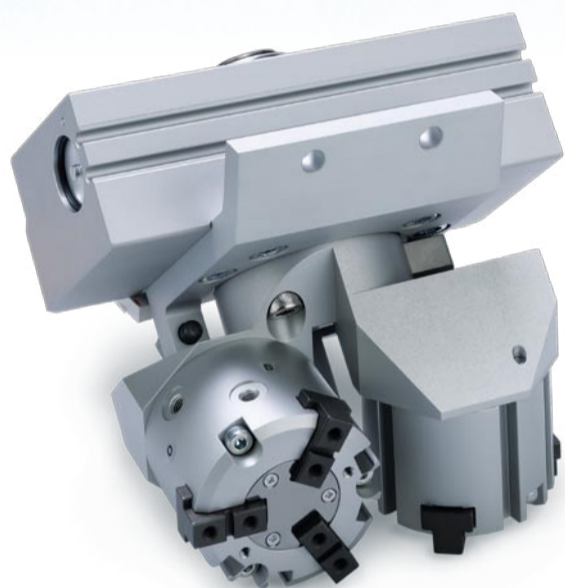
Double gripper reversing unit
